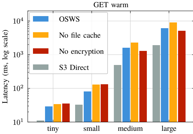
Fig. 5a. Median GET latency on warm cache
