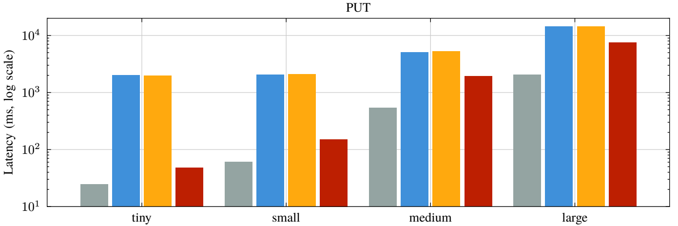
Fig. 5c. Median PUT latency
