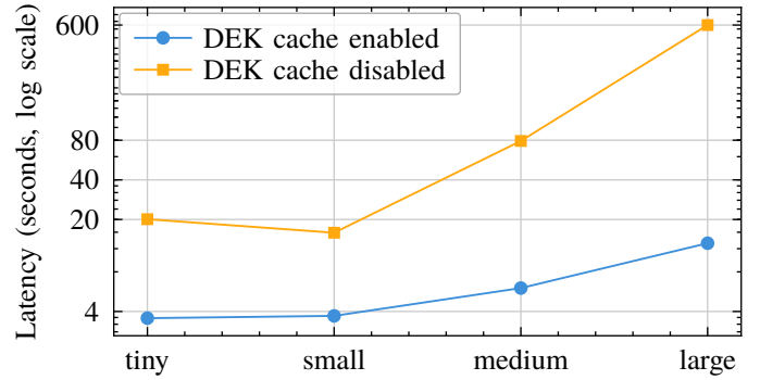
Figure 4. DEK cache impact on median cold GET latency. (logarithmic scale y axis)
