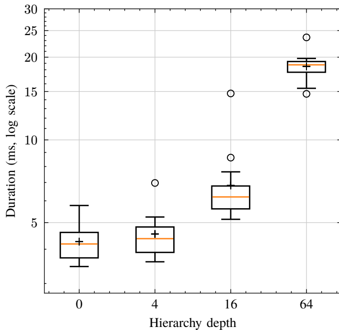
Fig. 3c. PermissionHierarchy box-plot distribution per parameter set (logarithmic y axis)
