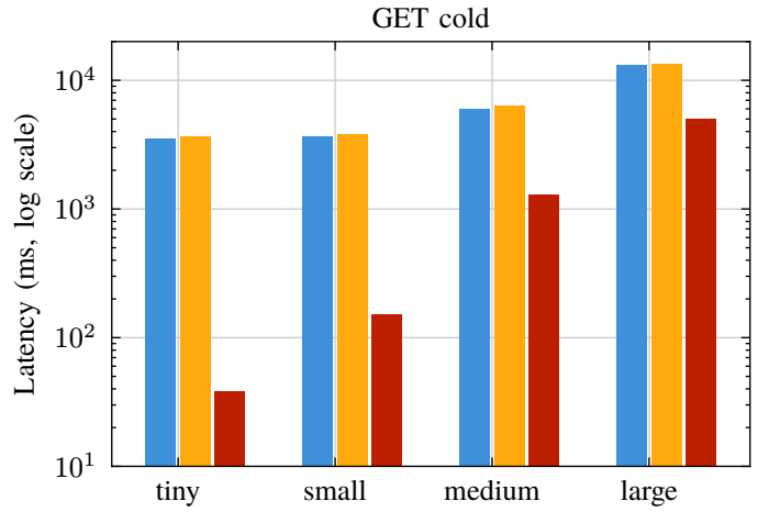
Fig. 5b. Median GET latency on cold cache
